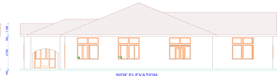
SIDE ELEVATION
